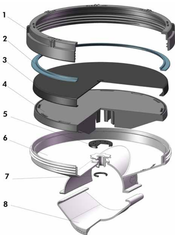
iDISC®-Aeration System: exploded view
